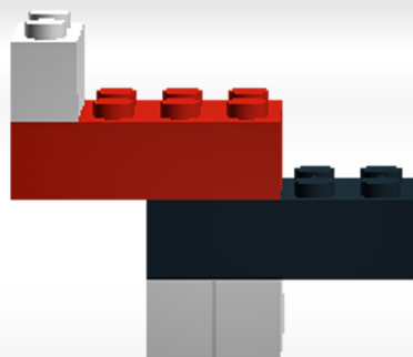
1 CH 2 OH group
