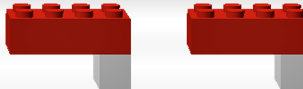
2 OH groups with H pointing down
