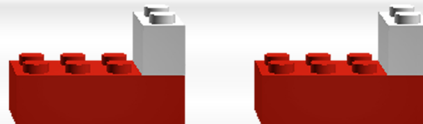
2 OH groups with H pointing up
